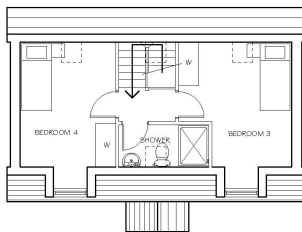
SECOND FLOOR PLAN PLOTS 14, 16 & 32
