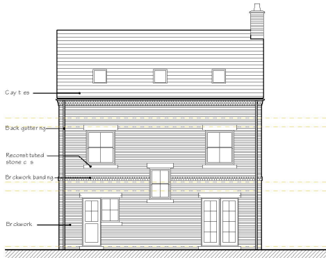
REAR ELEVATION PLOTS 14, 16 & 32
