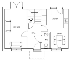
GROUND FLOOR PLAN PLOTS 14, 16 & 32
