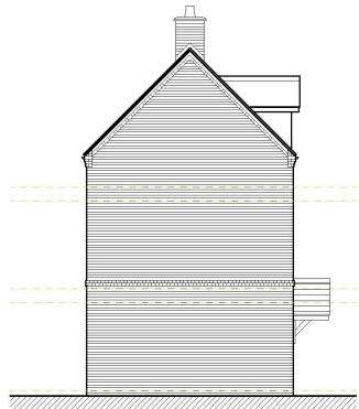
SIDE ELEVATION PLOTS 14, 16 & 32
